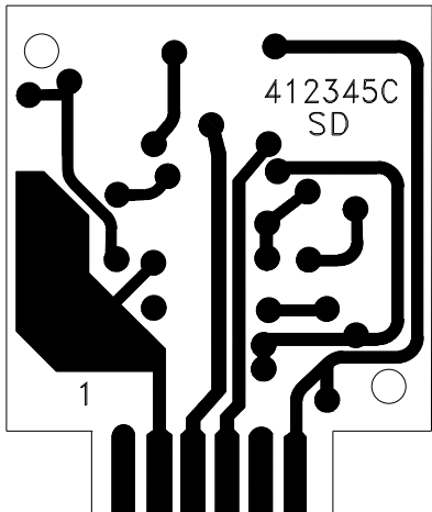
Layout as it would appear when applied to blank PCB.
