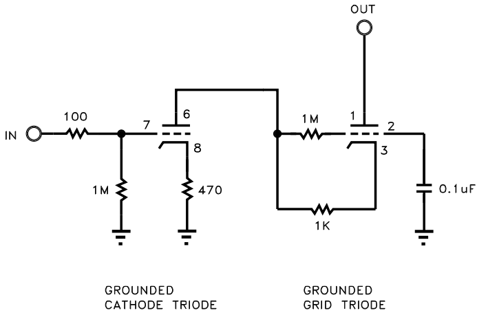
SCHEMATIC
