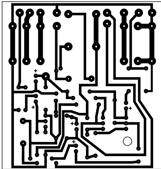
SCHALLER "BOW WOW YOY YOY" PCB LAYOUT BY PAUL MAROSSY 9/4/06
