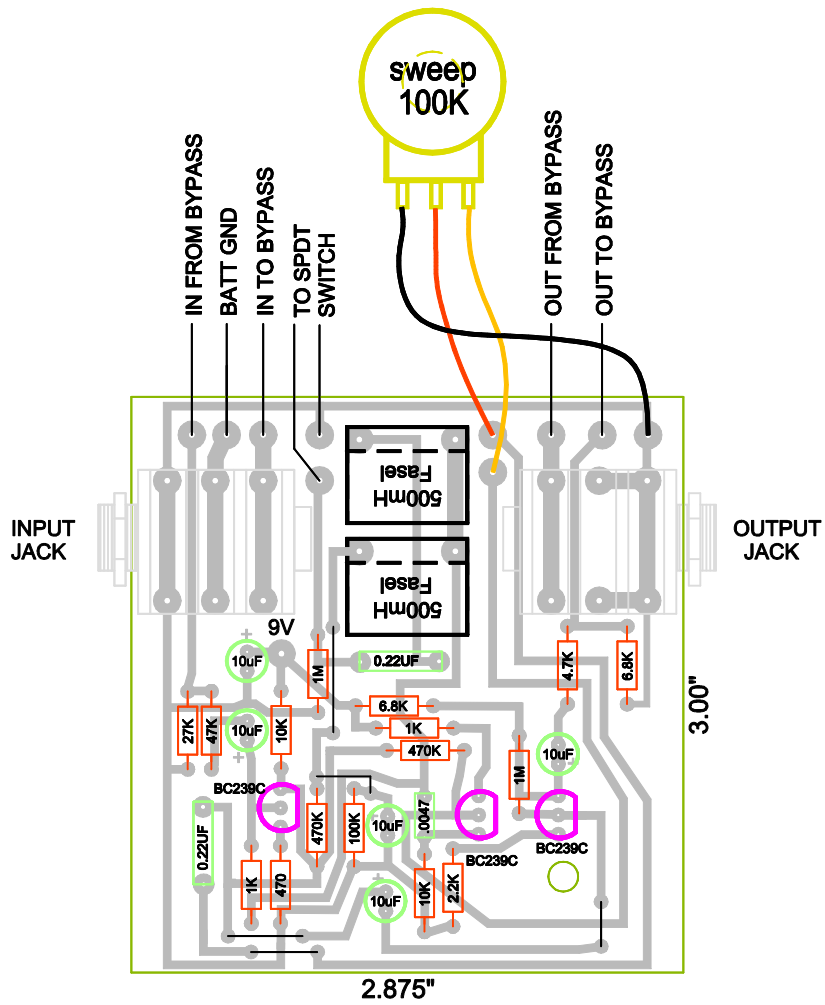
SCHALLER "BOW WOW YOY YOY" PCB LAYOUT BY PAUL MAROSSY 9/4/06
